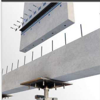
NXT™ Precast Panel on strip footing
