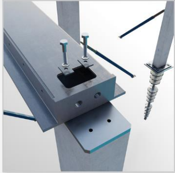
NXT™ Beam on NXT™ Column
