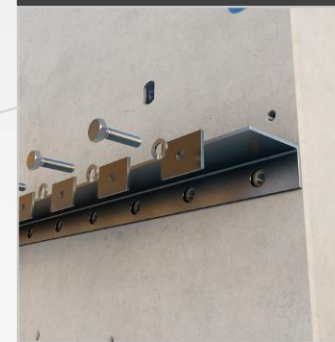
NXT™ Precast Panel with angle line
